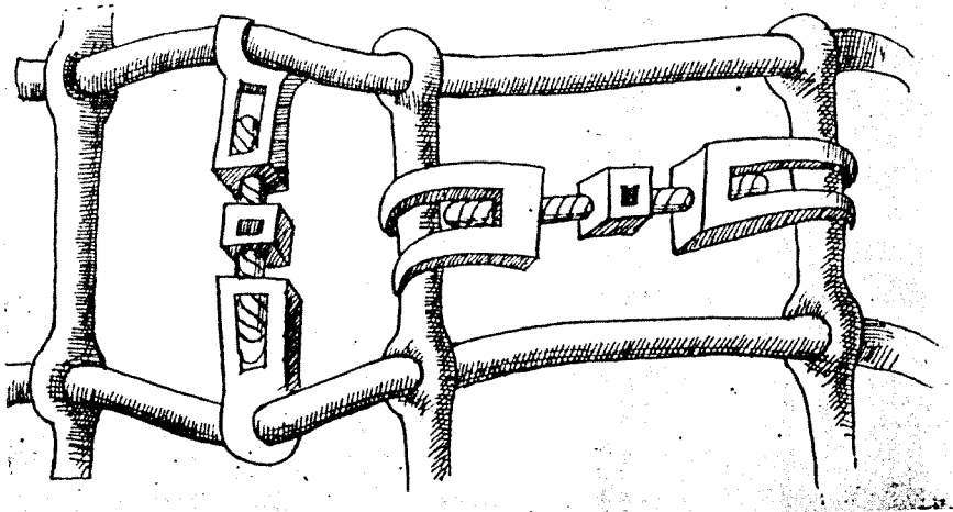
Figure 4.28 Copyist's version of drawing by Francesco di Giorgio.
